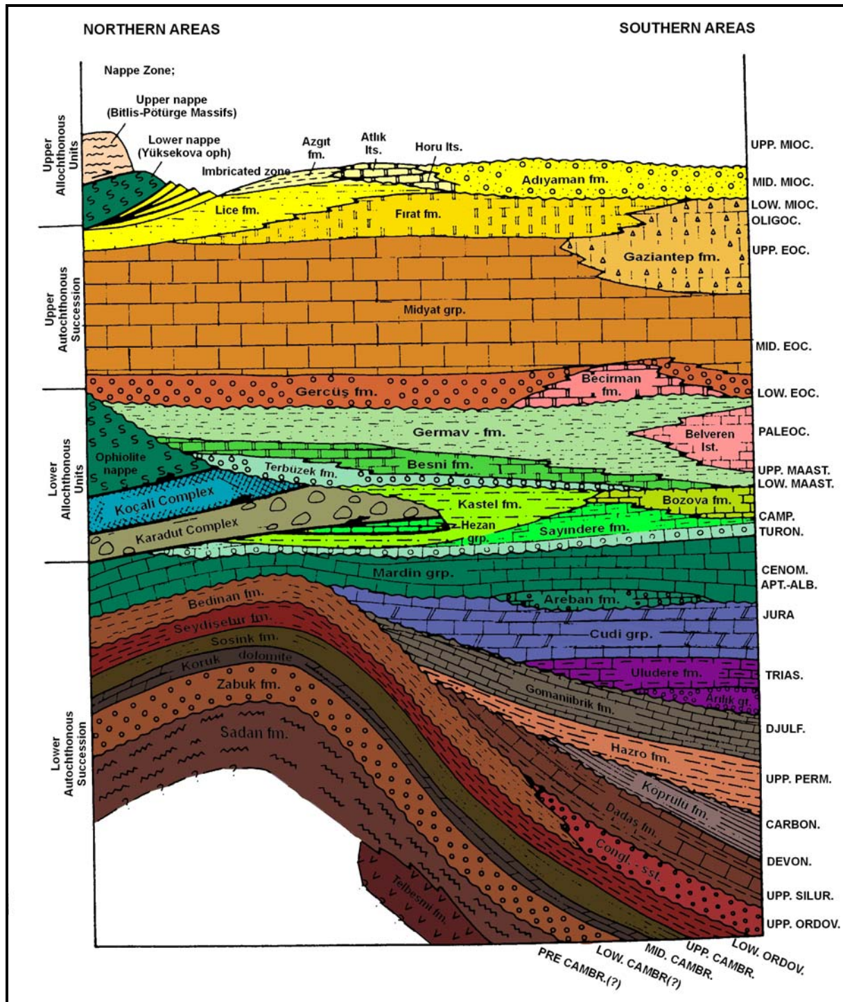
Stratigraphic units of Southeast Turkey
