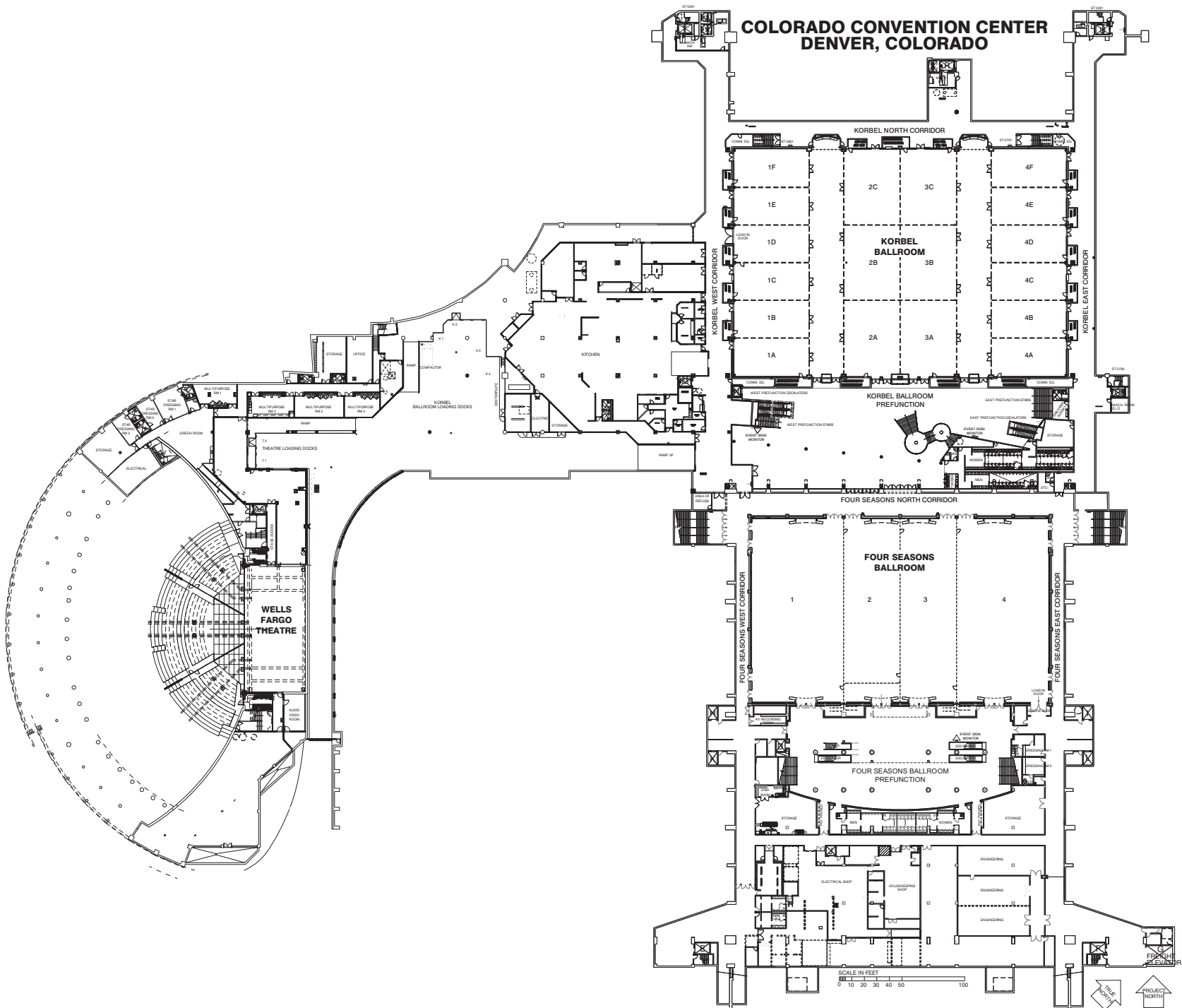
OVERALL PLAN - LOWER LEVEL BALLROOM/THEATRE LEVEL
