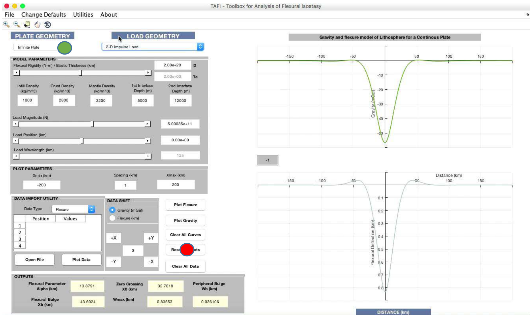
Figure 3. Toolbox for Analysis of Flexural Isostasy (TAFI) graphical user interface (GUI). When viewed in the PDF of this paper using Adobe Acrobat or Reader, clicking on green circles activates a dynamic figure demonstrating GUI features. These include (1) available plate geometry (pull-down menu); (2) available load geometry (pull-down menu); (3) changing the flexural rigidity (slider); and (4) changing the load magnitude (slider). Clicking on the red circle resets the figure to its initial display. Other model parameters controlled with sliders and text boxes are the load position, load wavelength for harmonic loads, and plate density structure (infill density, crust density, mantle density, and the respective interface depths). Plot appearance is controlled with “Xmin”, “Xmax”, and “Spacing” in the “Plot Parameters” panel. Flexure or gravity data can be imported using the “Data Import Utility”, which prompts for an input file name. The data are plotted by clicking the “Plot Data” button. X, Y, and Z buttons and edit box in the “Data Shift” panel allow data to be shifted horizontally and vertically to adjust the model fit. Buttons to interact with the imported data and plots are also provided. The flexural parameter ( \alpha [indicated as Alpha in the TAFI GUI]), zero crossing distance ( x_0 [X0 in the GUI]), flexural bulge position ( x_b [Xb in the GUI]), the maximum flexural depth ( w_{max} [Wmax in the GUI]) and the amplitude of peripheral bulge ( w_b [Wb in the GUI]) are displayed in the “Outputs” panel. Flexure and gravity models and imported data are shown in the plot panel.
